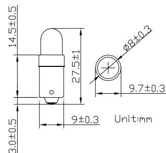
Outline Dimension
