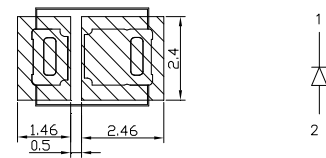
Recommended Solder Pad
