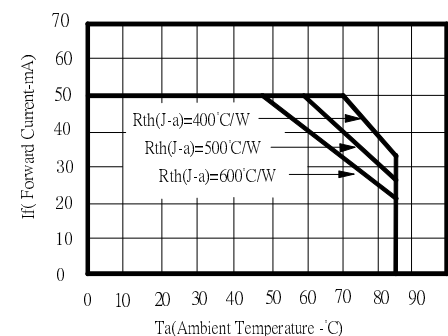
Maximum Permissible Forward Current T J =115°C
