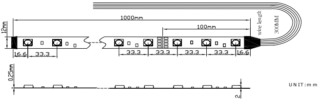
Outline Dimension
