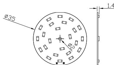
Outline Dimension
